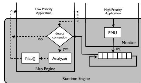
Figure 4. ReQoS Runtime Architecture
